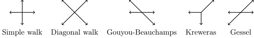
Figure 2: Some famous models of planar walks. The first two ones are solved in the three-quadrant in [11]
