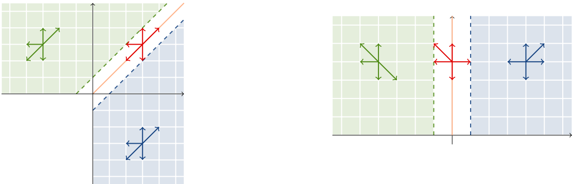
Figure 4: Solving a walk model in the three-quadrant cone is equivalent to solving a space inhomogeneous model in a half-plane
