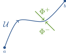
Figure 15: Left and right limits on the open contour \mathcal{U}
